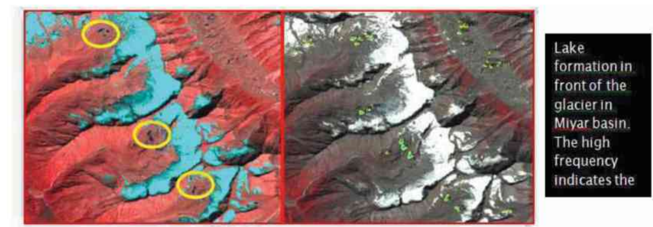
Moraine Dammed Lake Formation at the Glacier Snout in Miyar Basin
