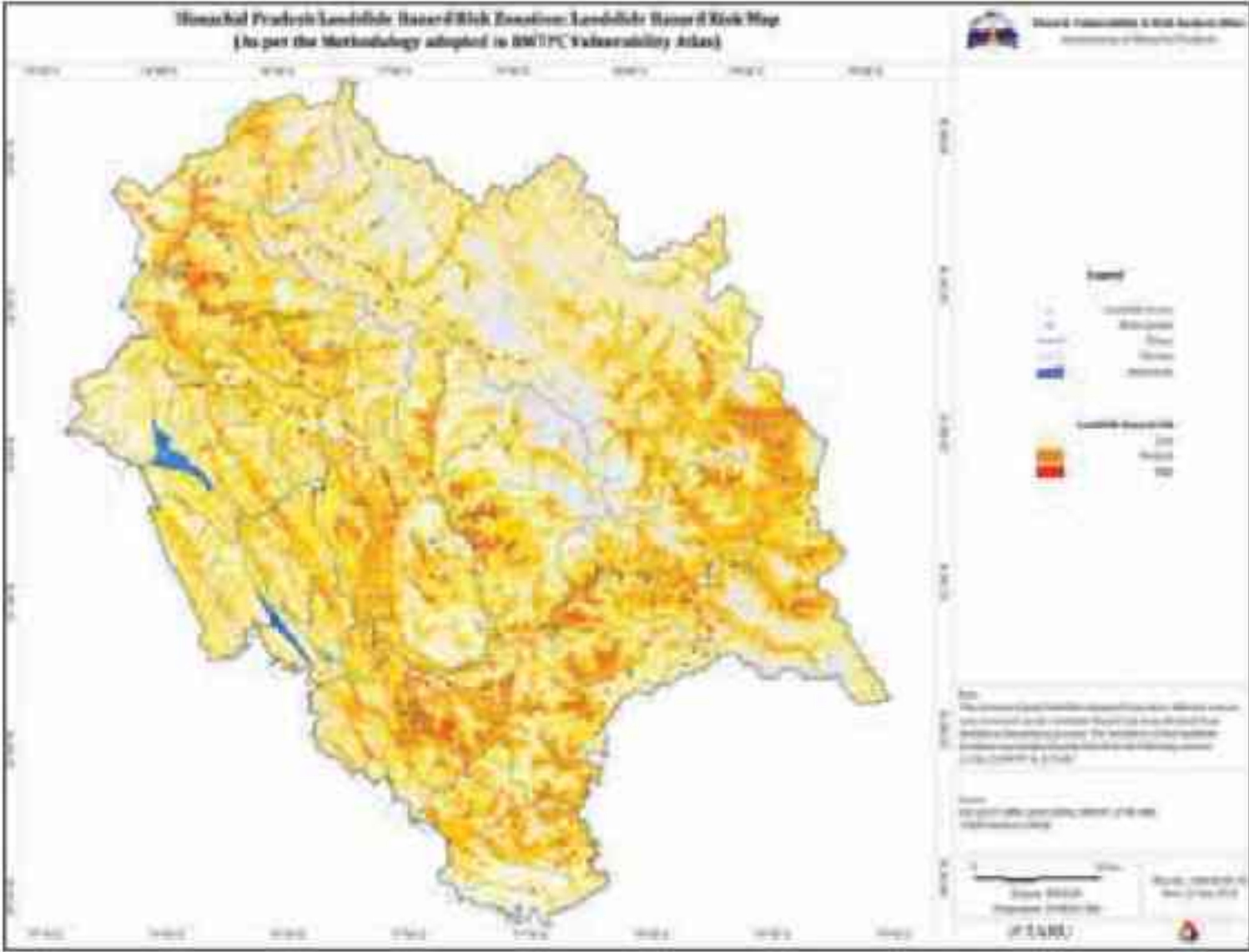
Map: Himachal Pradesh Land slide Hazard risk zonation
