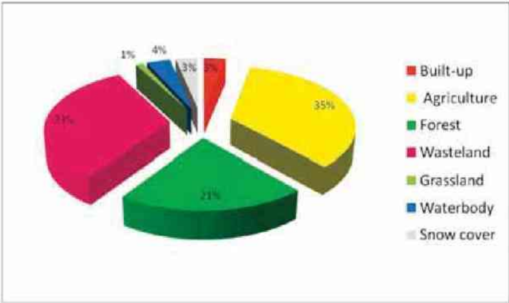
Fig.3b.Percentage area under different major land use categories in Hamirpur district for the year 2015-16.
