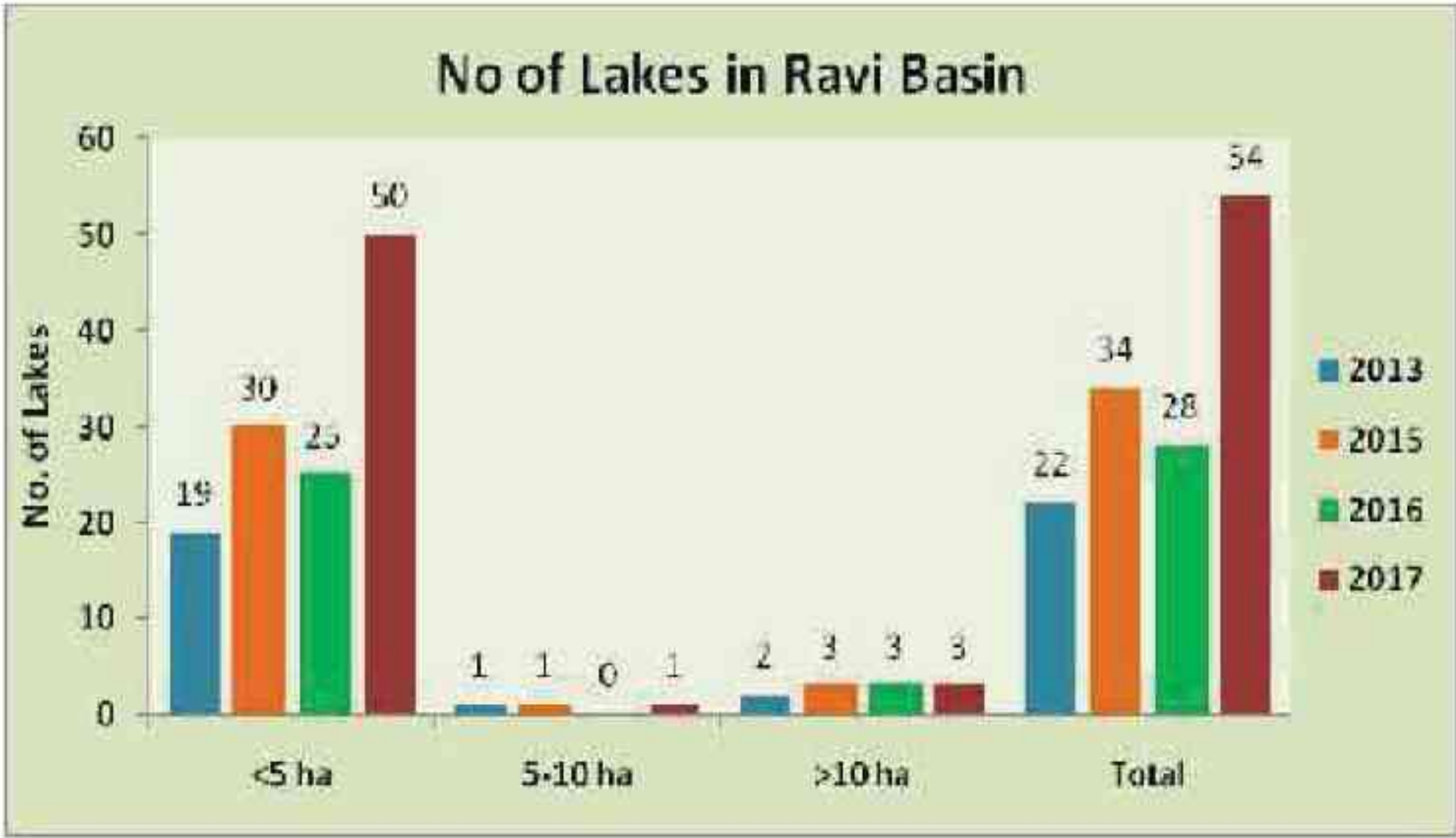
Fig.11.4 Distribution of lakes in Ravi basin
