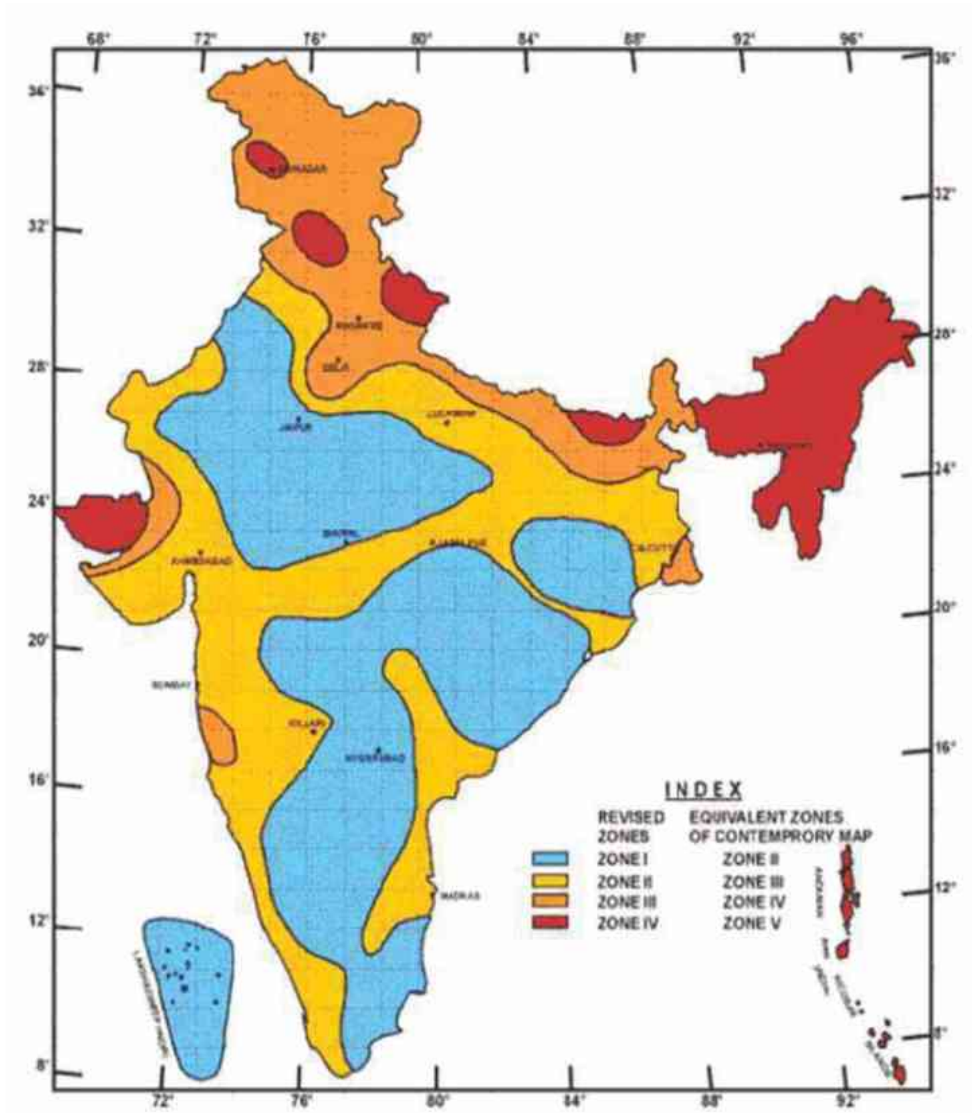
Seismic Zonation Map of India (As per Bureau of Indian Standards)
