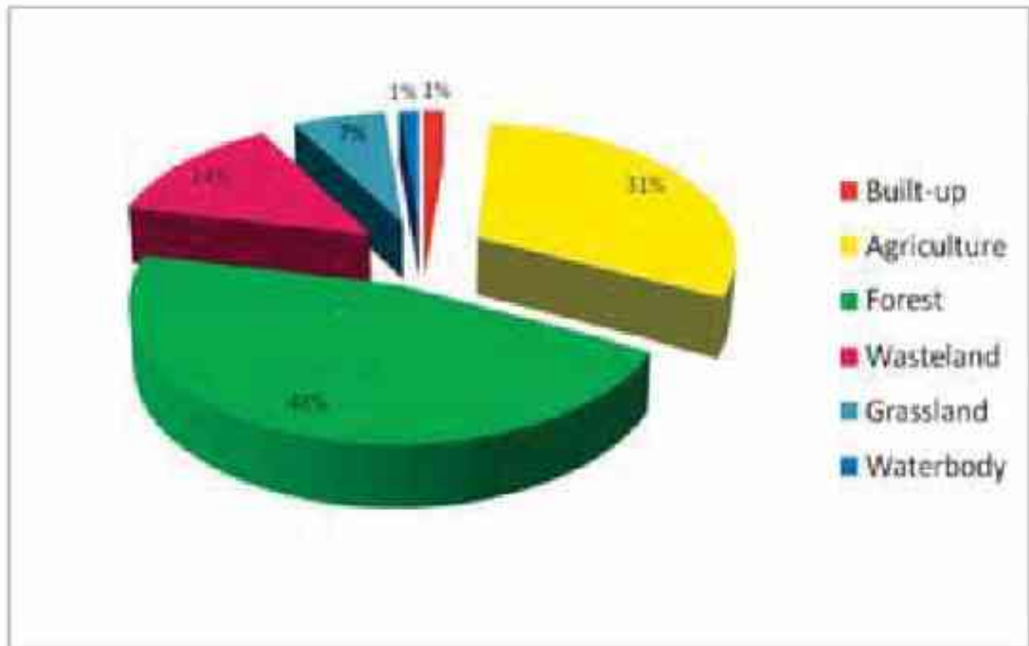
Fig. 1b. Percentage area under different major land use categories in Bilaspur district for the year 2015-16.
