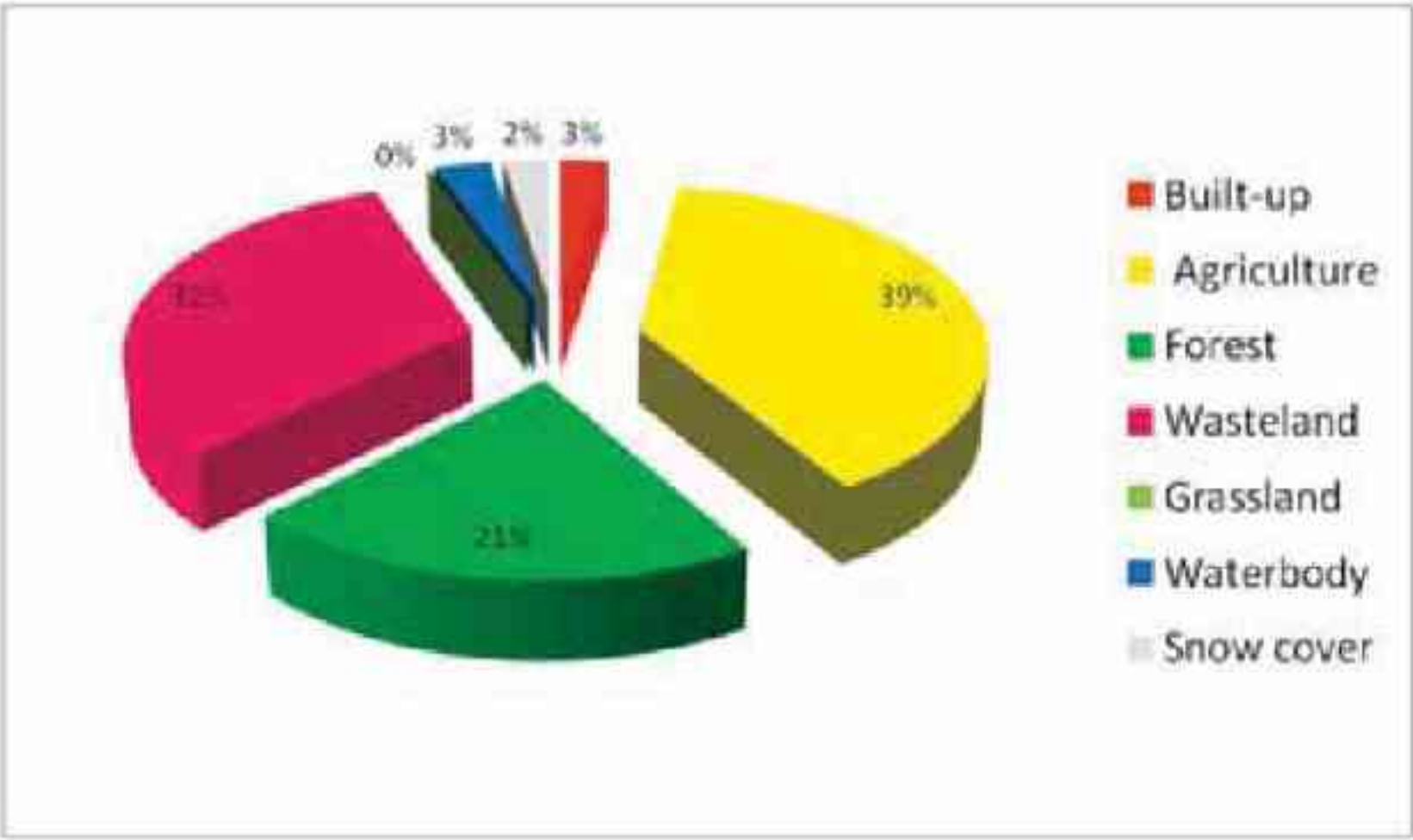
Fig. 3a. Percentage area under different major land use categories in Hamirpur district for the year 2005-06.
