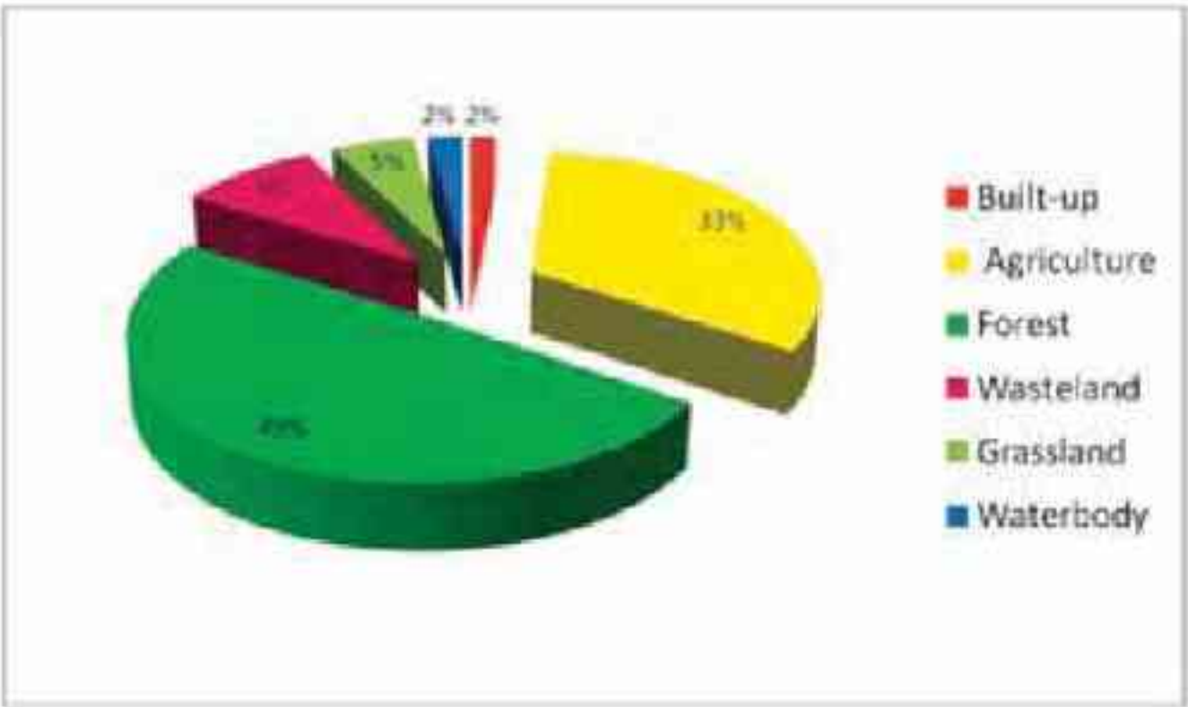
Fig.10a. Percentage area under different major land use categories in Sirmour district, 2005-06.
