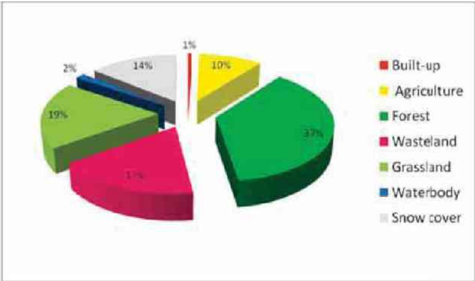
Fig. 2a. Percentage area under different major land use categories in Chamba district for the year 2005-06.
