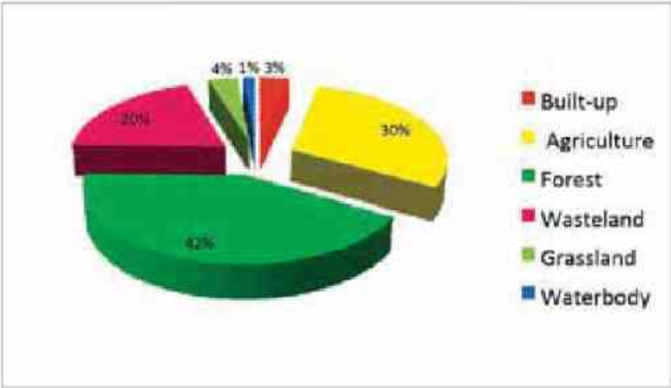
Fig.11a. Percentage area under different major land use categories in Solan district, 2005-06.
