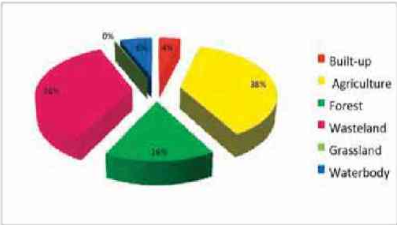
Fig. 12b. Percentage area under different major land use categories in Una district,2015-16.
