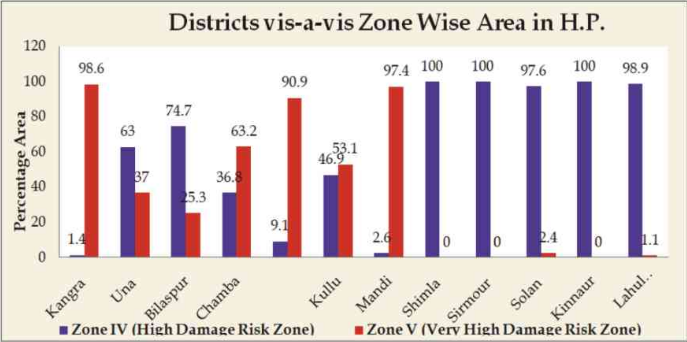
Districts vis-à-vis zone wise area in Himachal Pradesh
