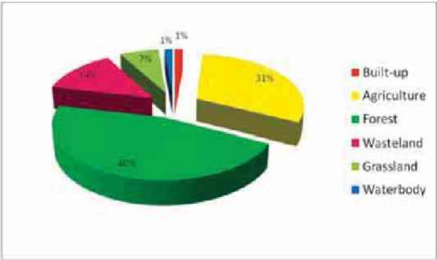
Fig. 8b. Percentage area under different major land use categories in Mandi district, 2005-06.
