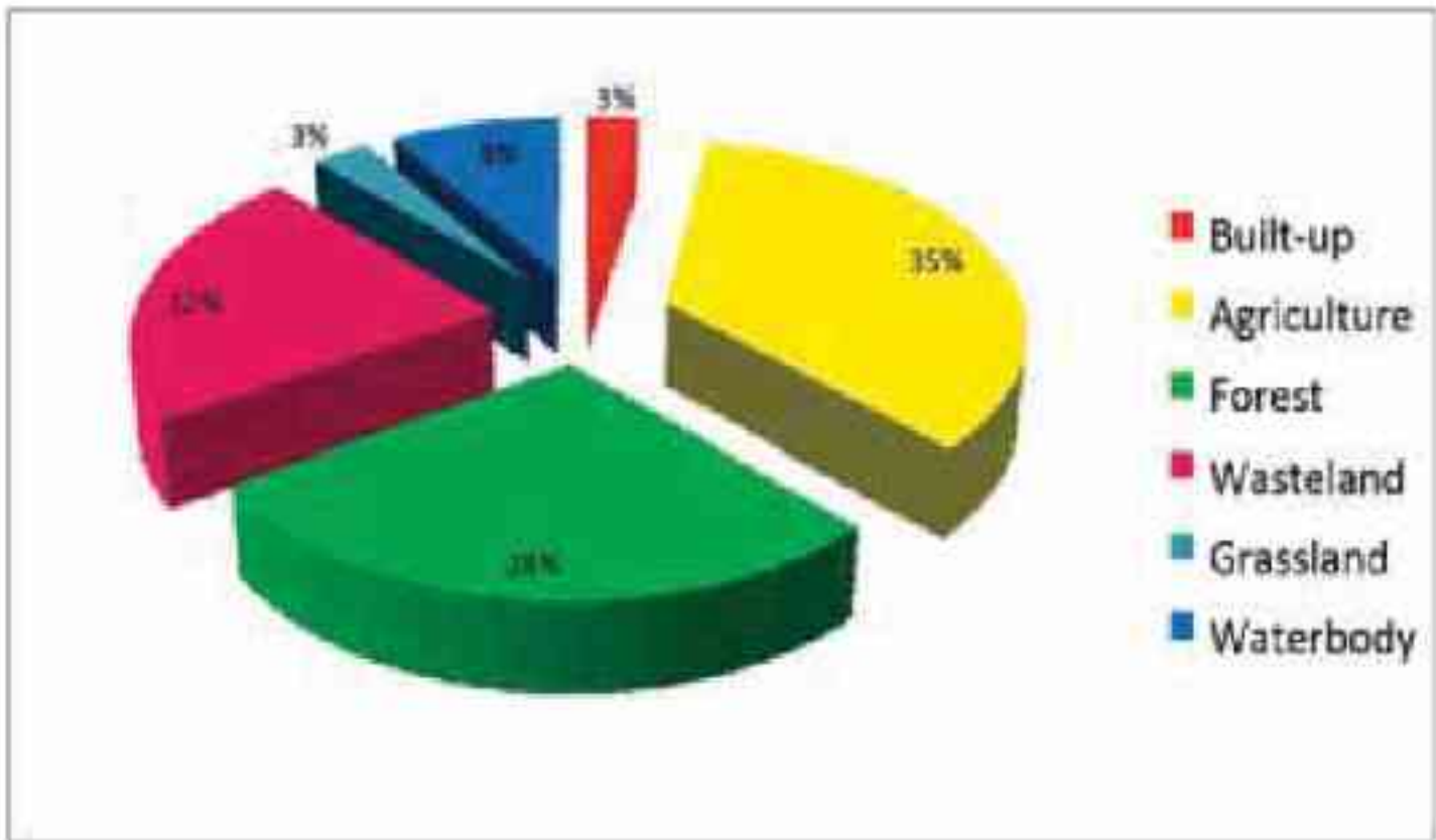
Fig. 1a. Percentage area under different major land use categories in Bilaspur district for the year 2005-06.
