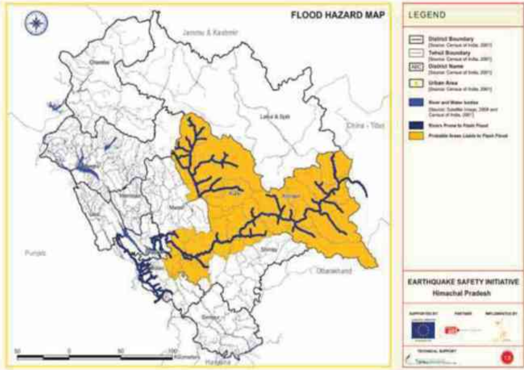
(Source: Vulnerability Atlas-SDMA ,H.P.) Rivers Prone for Flood Hazards in H.P.
