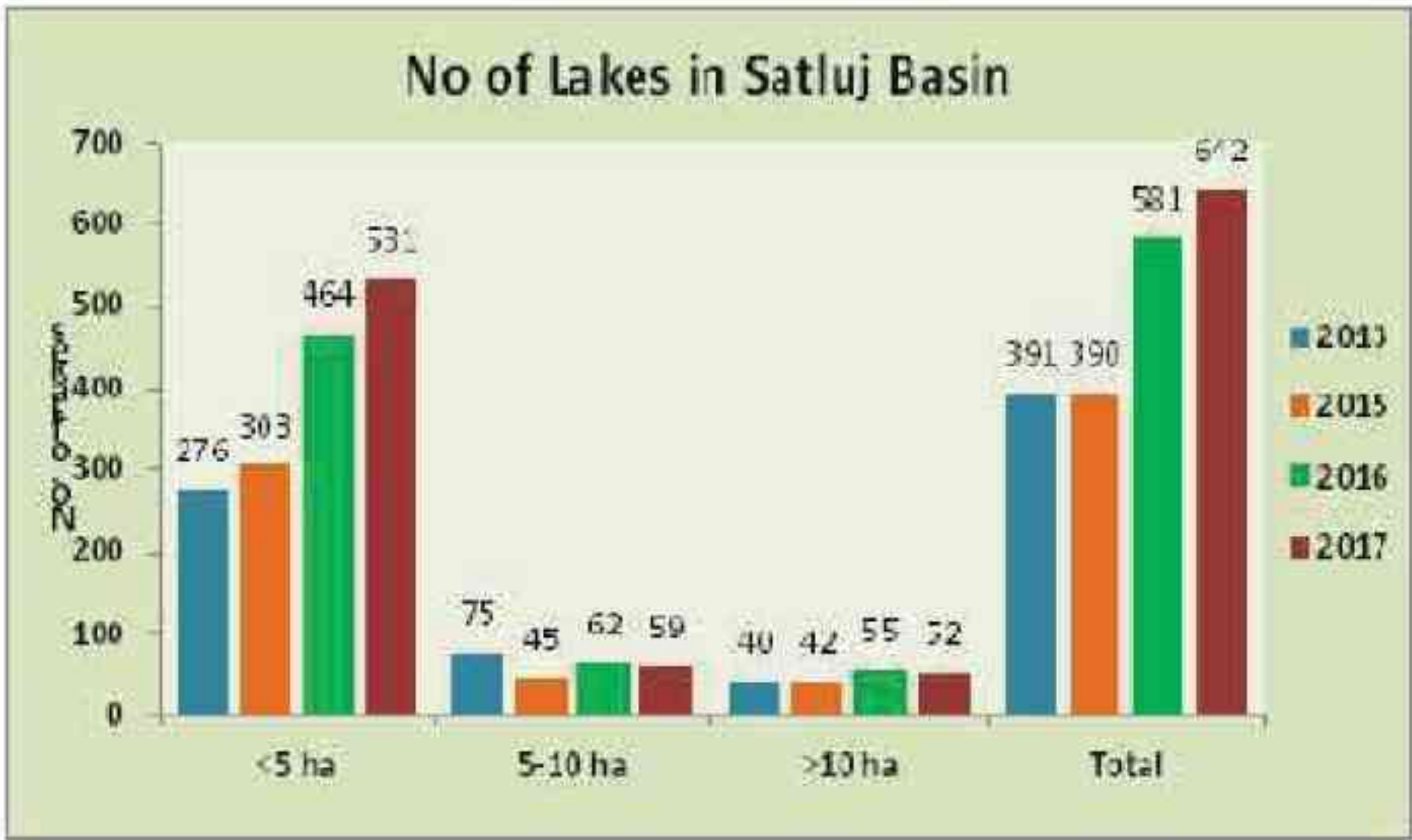
Fig.11.1 Distribution of lakes in Satluj basin
