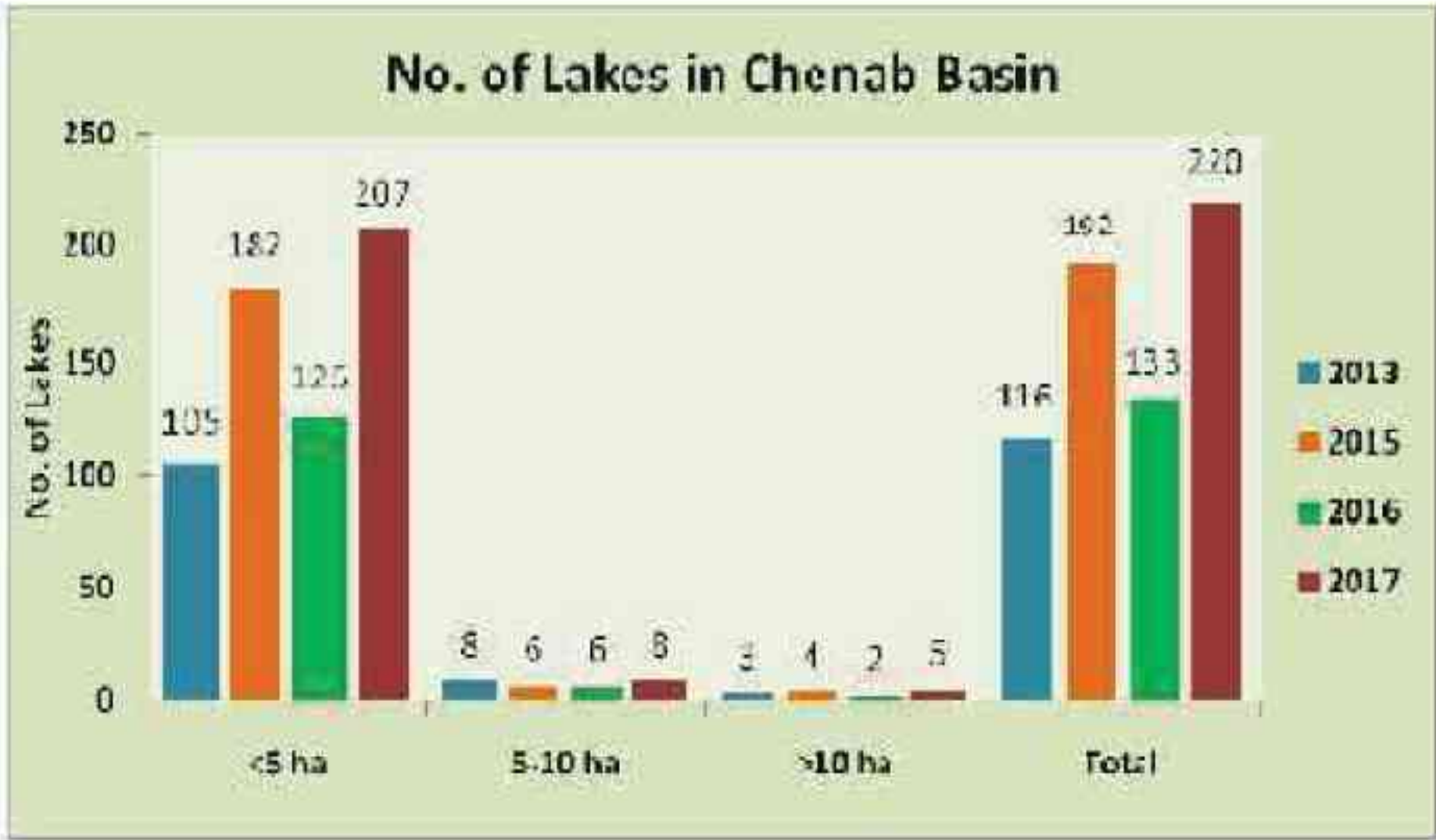
Fig.11.2 Distribution of lakes in Chenab basin
