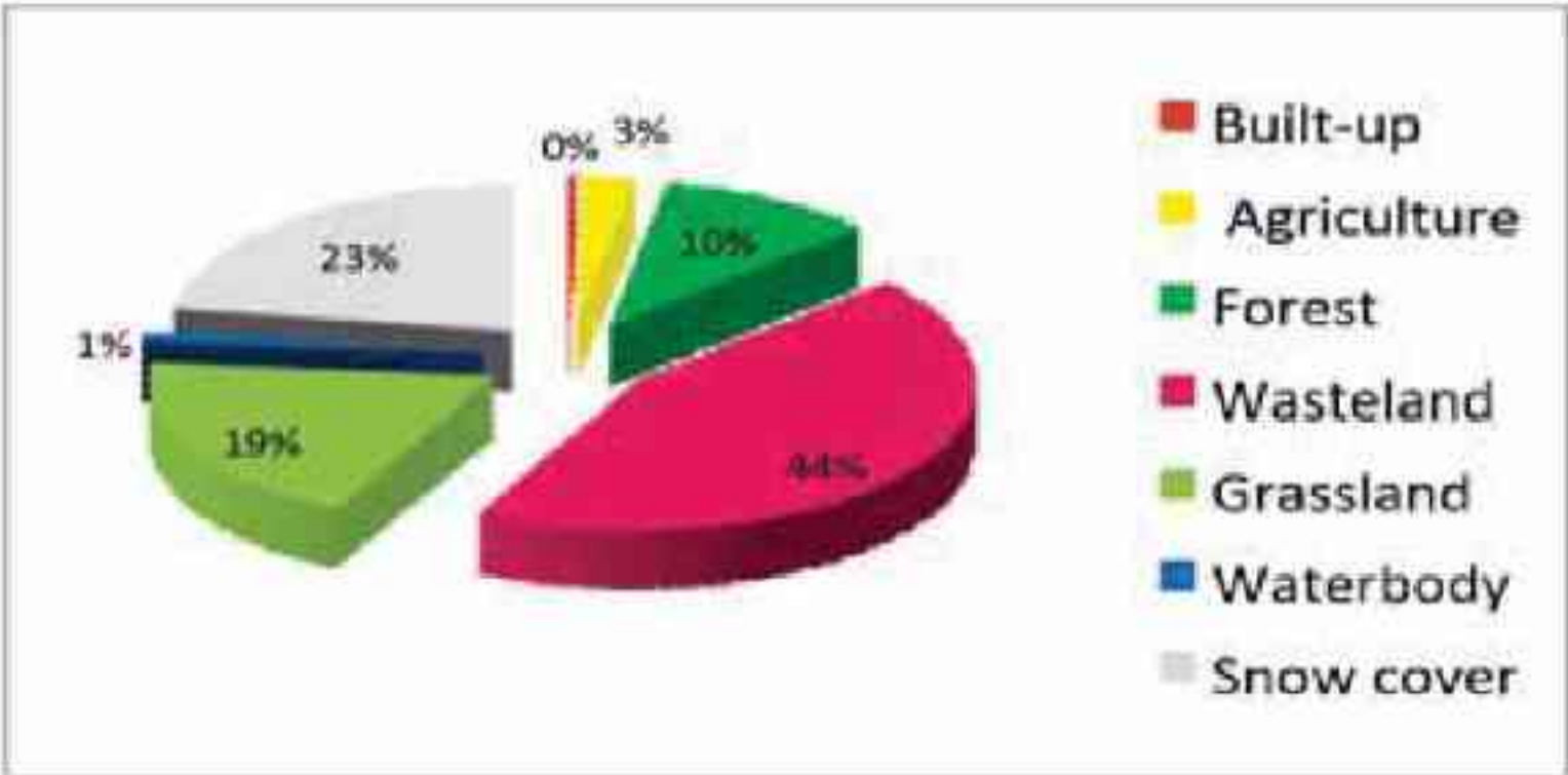
Fig. 5b. Percentage area under different major land use categories in Kinnaur district, 2015-16.
