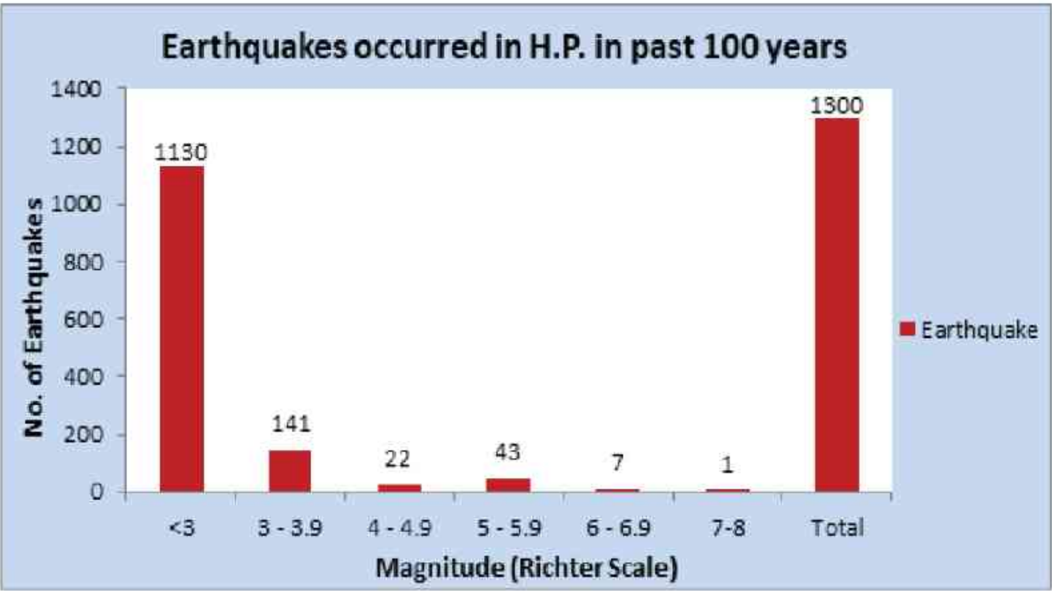
Graphical representation of earthquakes occurred in H.P. in past 100 year
