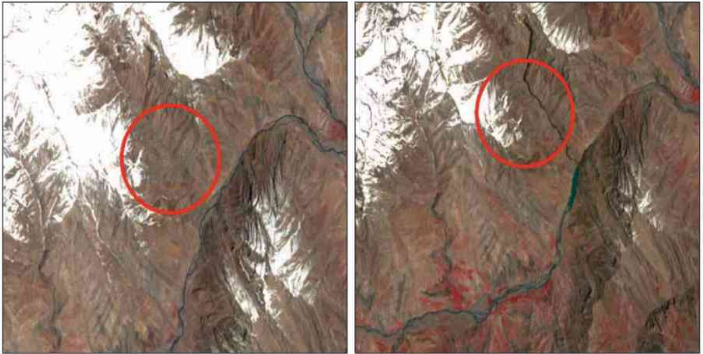
Debris Flow due to snowmelt along stream in Pin River Basin
