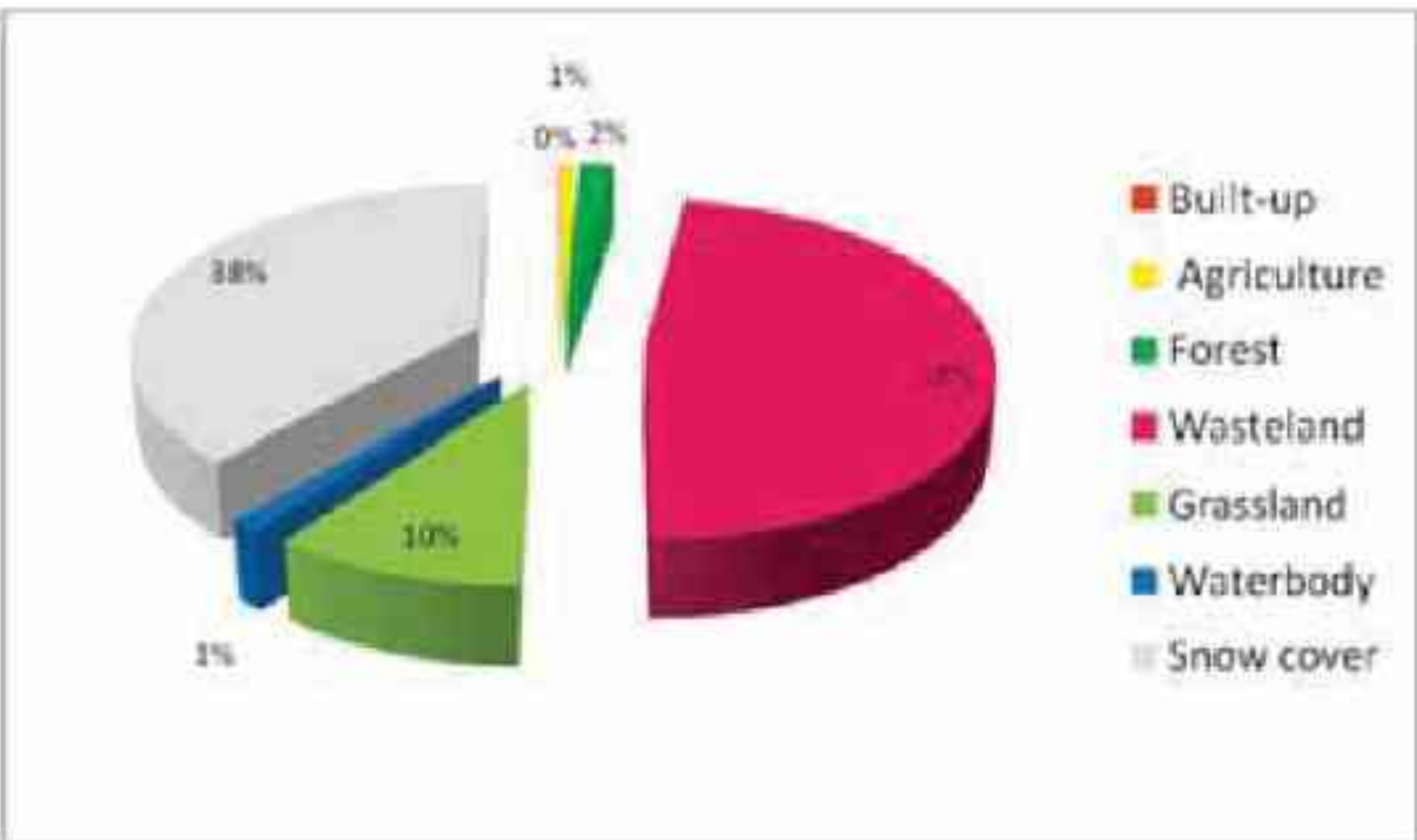
Fig. 7b. Percentage area under different major land use categories in Lahul-Spiti district 2015-16.
