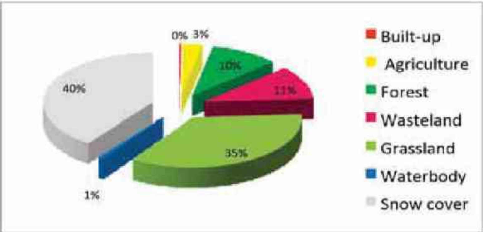
Fig. 5a. Percentage area under different major land use categories in Kinnaur district 2005-06.
