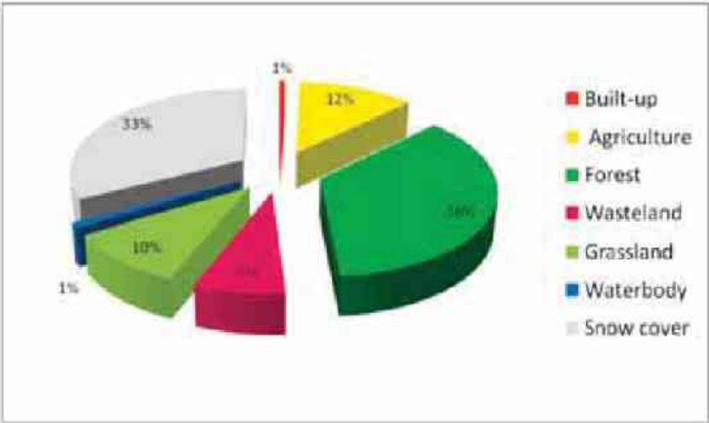
Fig. 6a. Percentage area under different major land use categories in Kullu district 2005-06.
