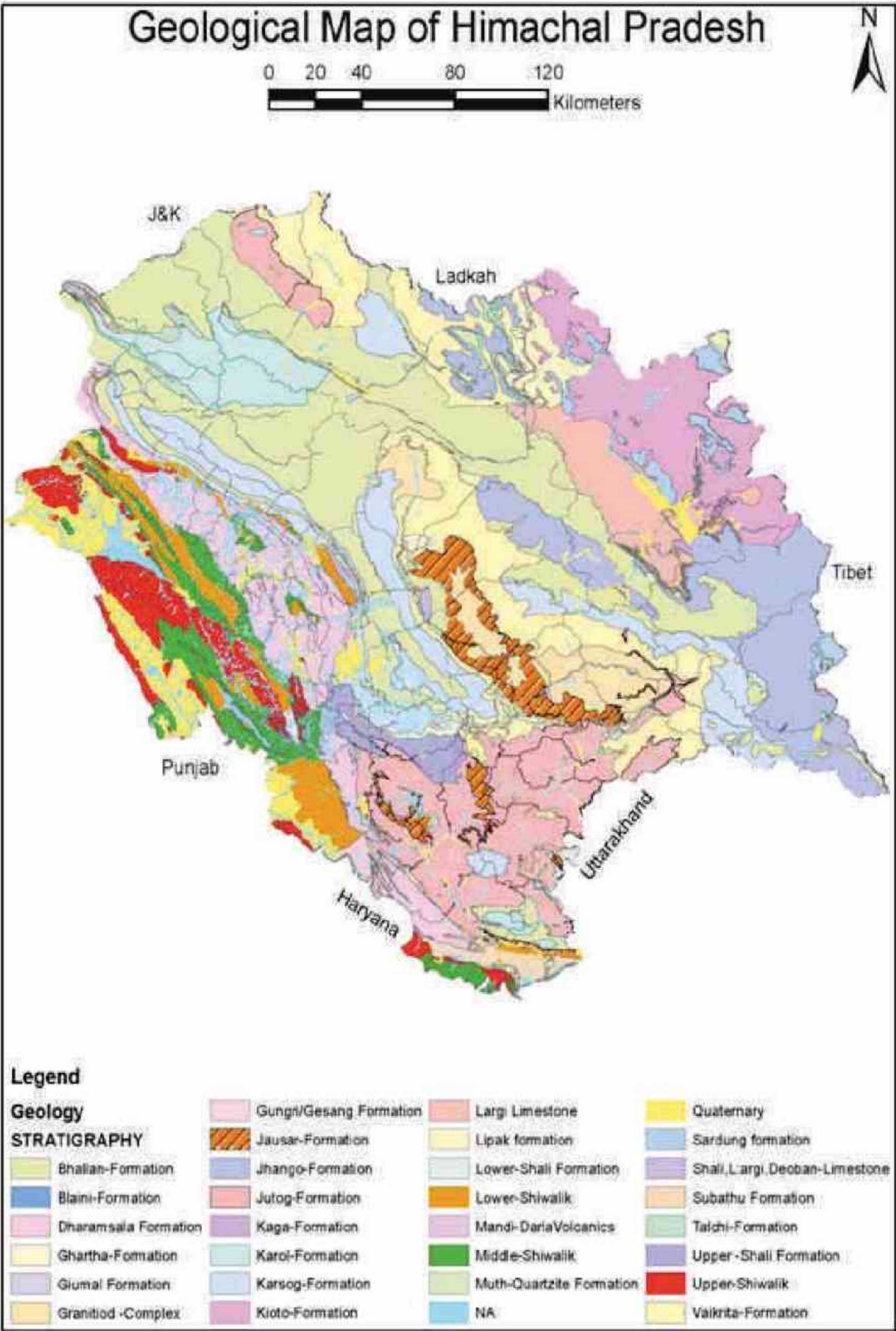
GeologicalMap of Himachal Pradesh (compiled based on published Literature by HIMCOSTE)
