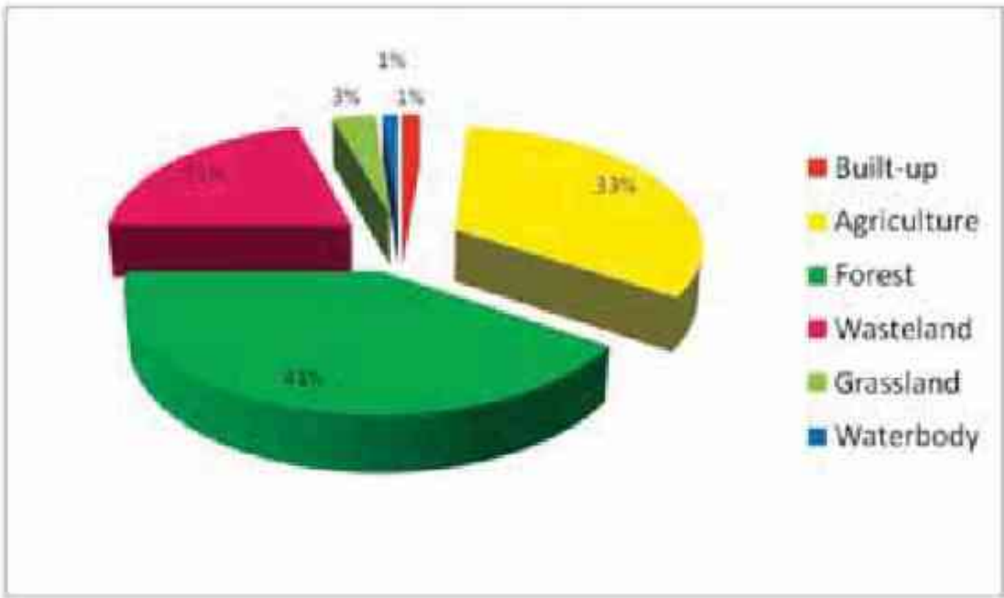
Fig. 8a. Percentage area under different major land use categories in Mandi district, 2005-06.
