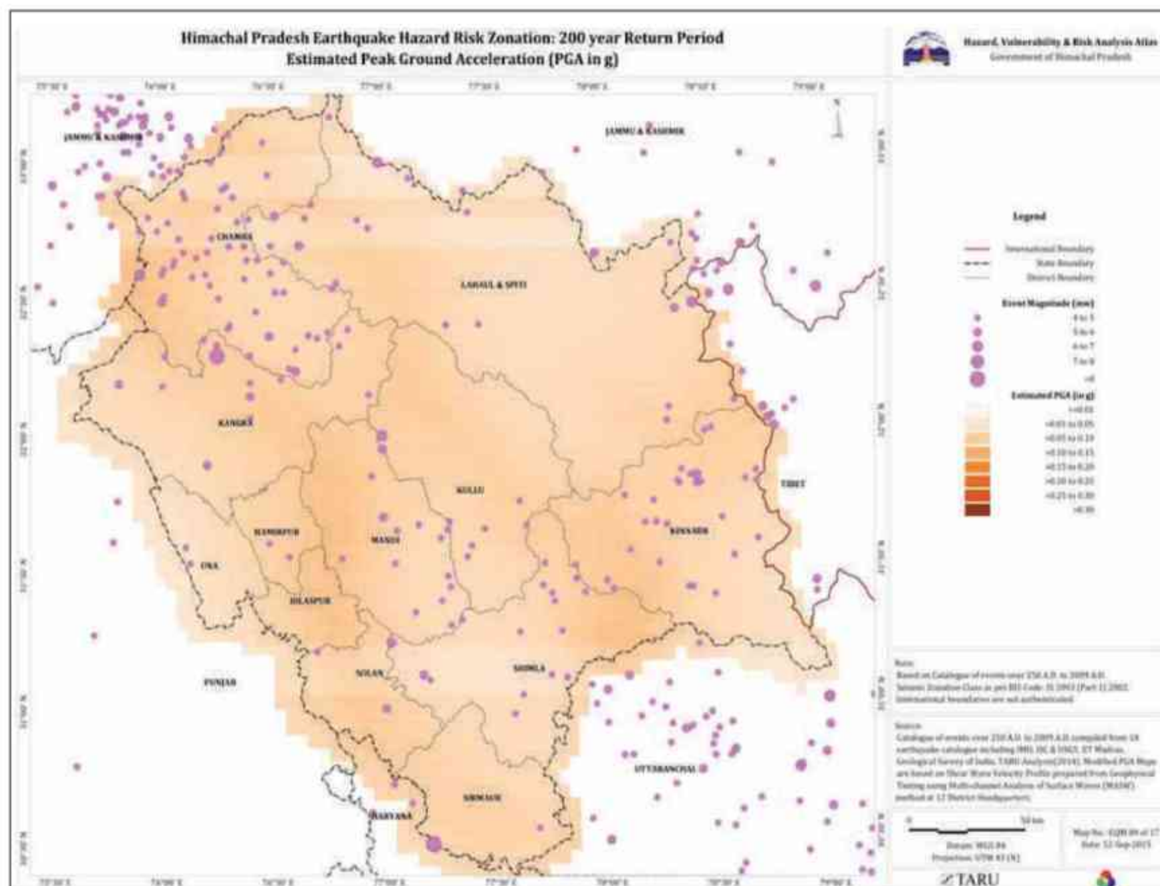
H. P. Earthquake Hazard Risk Zonation
