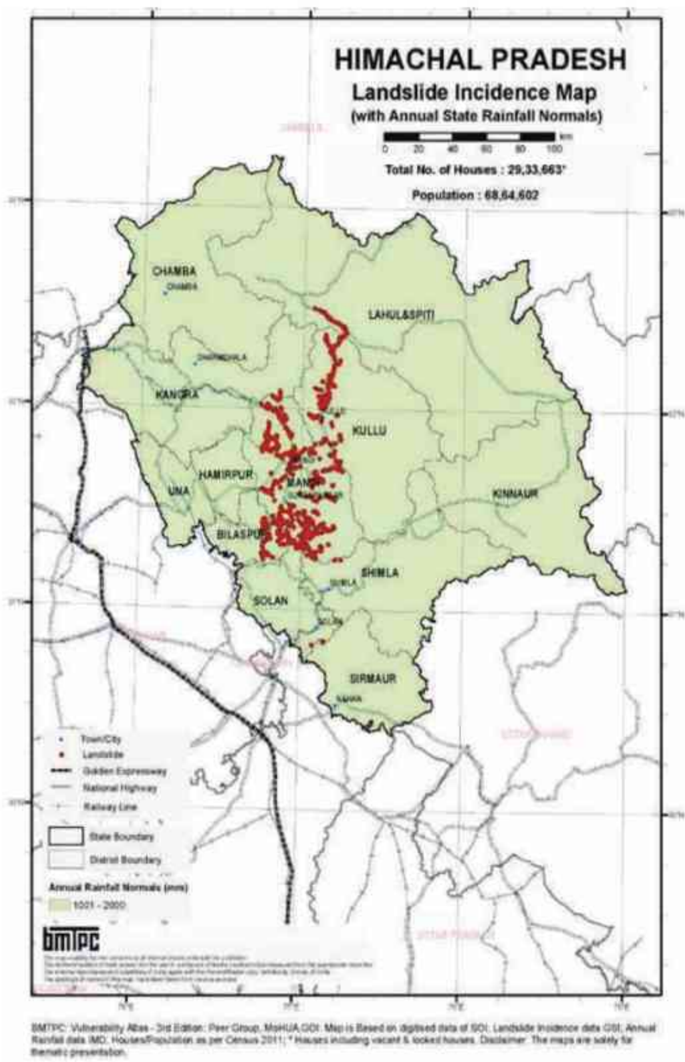
Landslide Incidence Map
