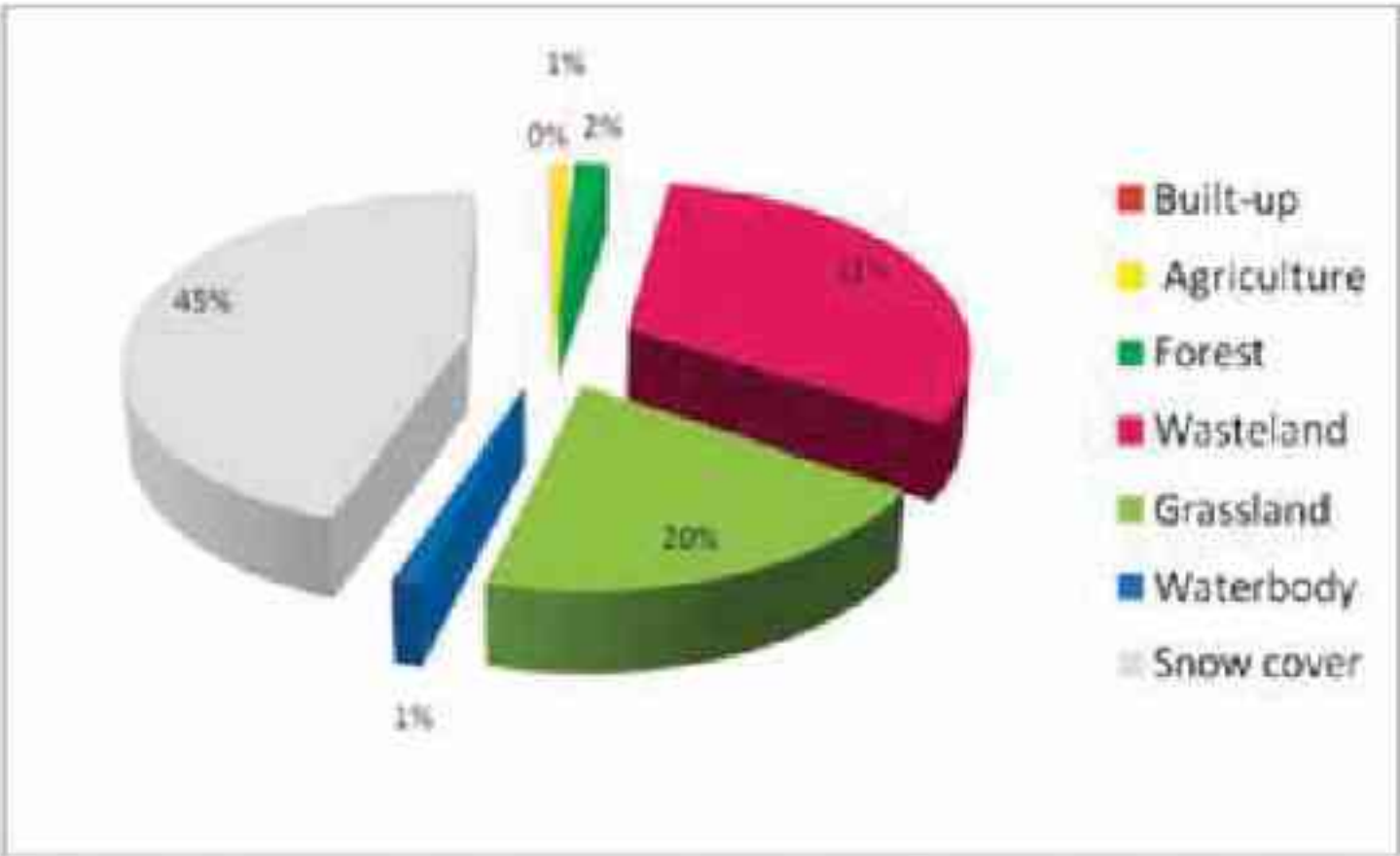
Fig. 7a. Percentage area under different major land use categories in Lahul-Spiti district 2005-06.
