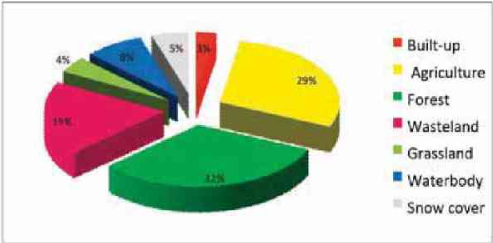
Fig. 4b. Percentage area under different major land use categories in Chamba district for the year 2015-16.
