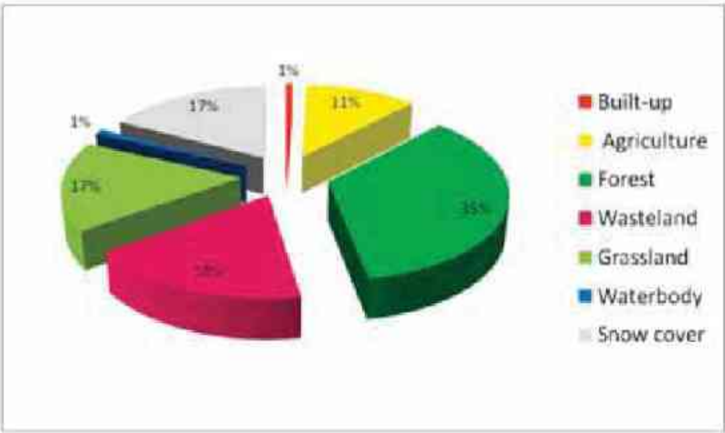
.Fig. 6b. Percentage area under different major land use categories in Kullu district 2015-16
