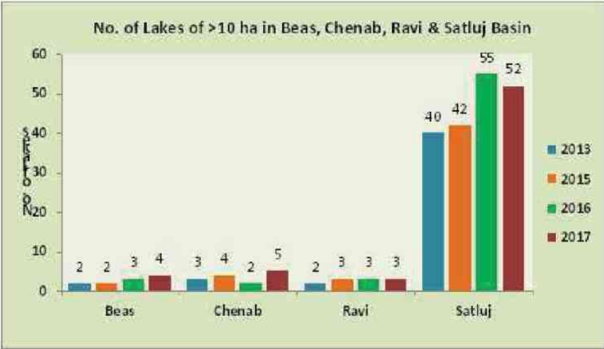
Fig.12.1 Distribution of lakes with area > 10 Ha in Chenab, Beas, Ravi & Satluj basin in 2013, 2015, 2016 & 2017
