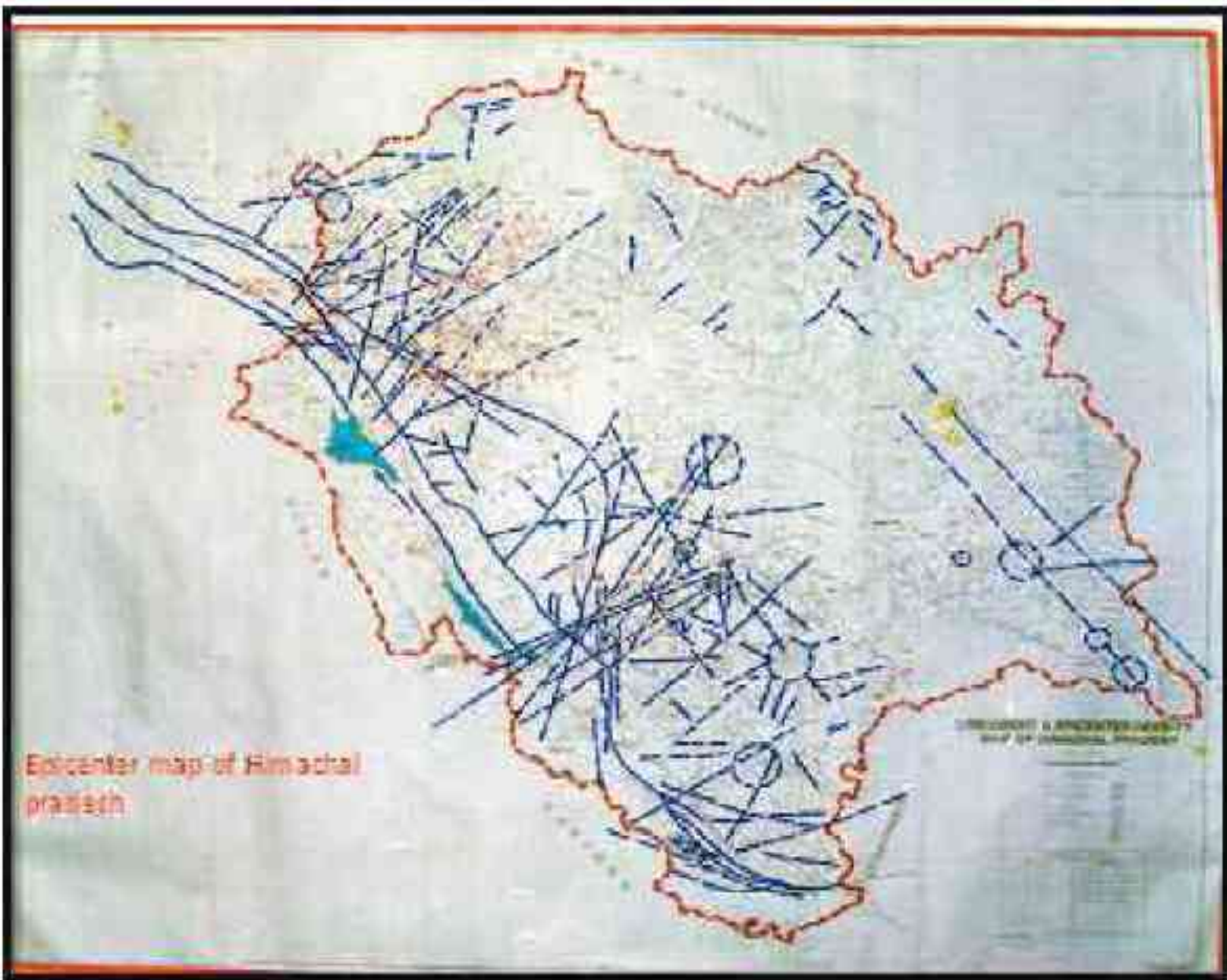
Epicentre Map of HP
