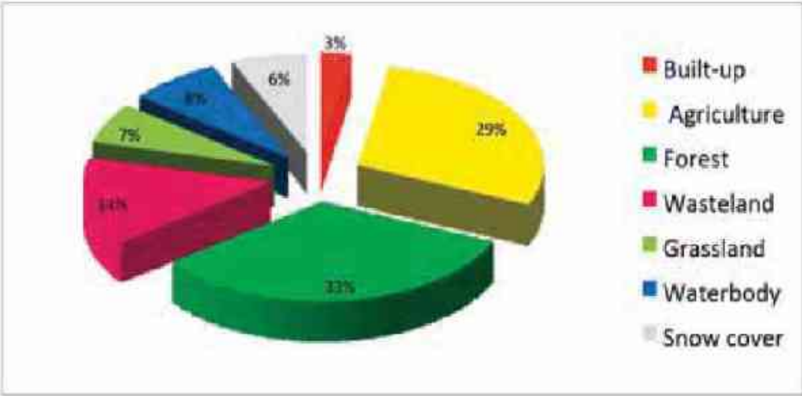
Fig. 4a. Percentage area under different major land use categories in Kangra district for the year 2005-06.
