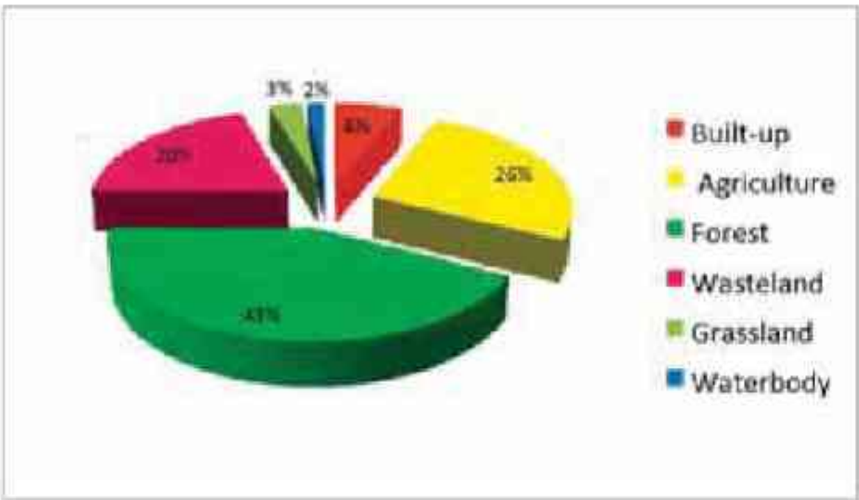
Fig. 11b. Percentage area under different major land use categories in Solan district, 2015-16.
