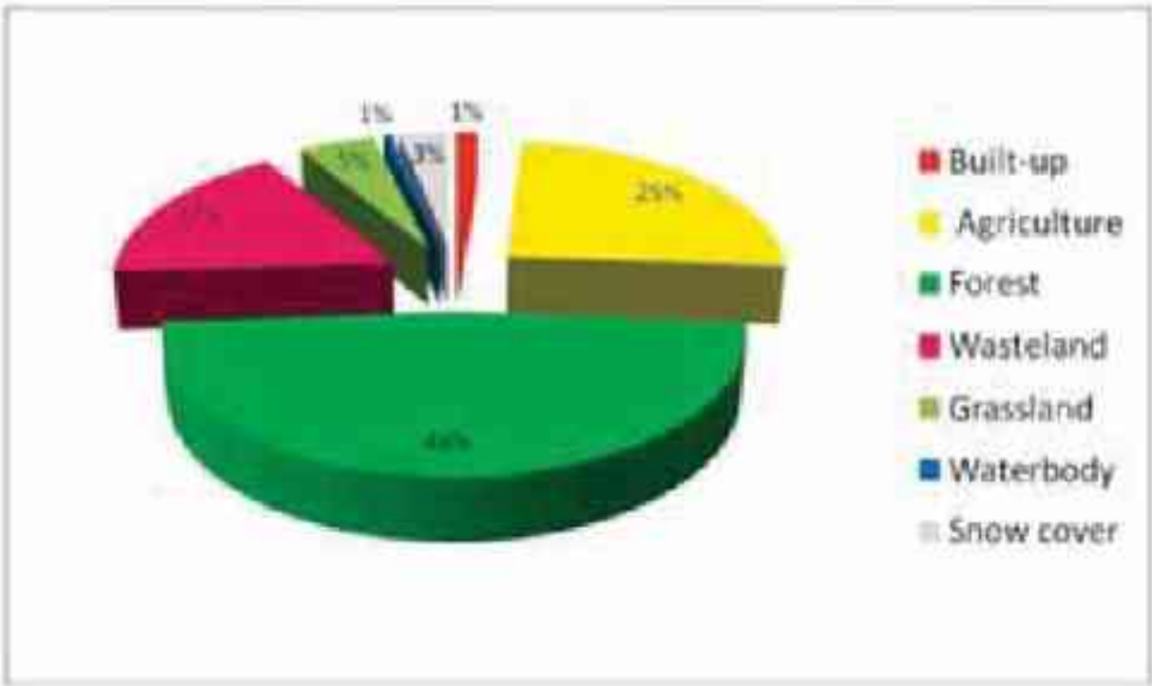
Fig. 9a. Percentage area under different major land use categories in Shimla district, 2005-06.
