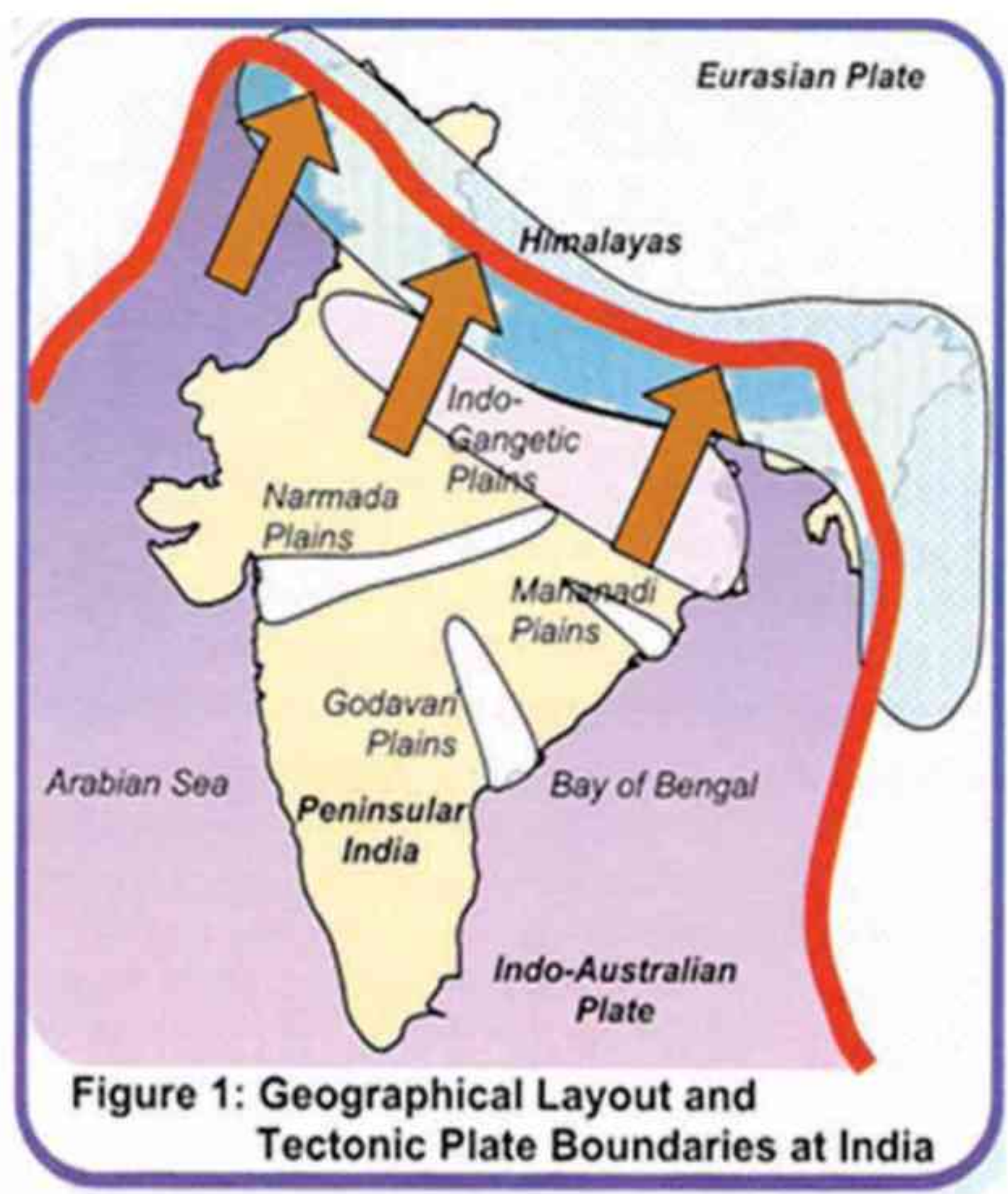
Geographical Layout and Tectonic Plate Boundaries at India
