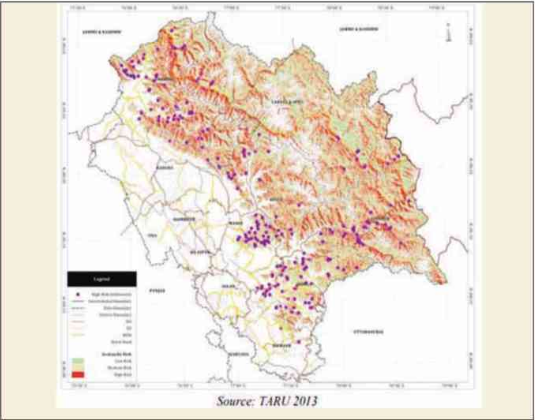
Avalanche Probability Zones, Himachal Pradesh
