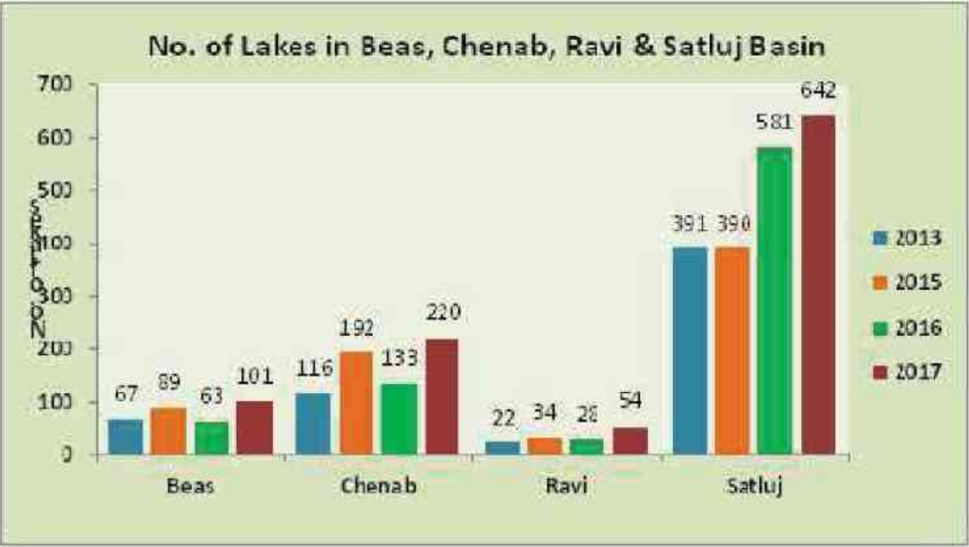
Fig.11.5 Distribution of lakes in Chenab, Beas, Ravi & Satluj basin
