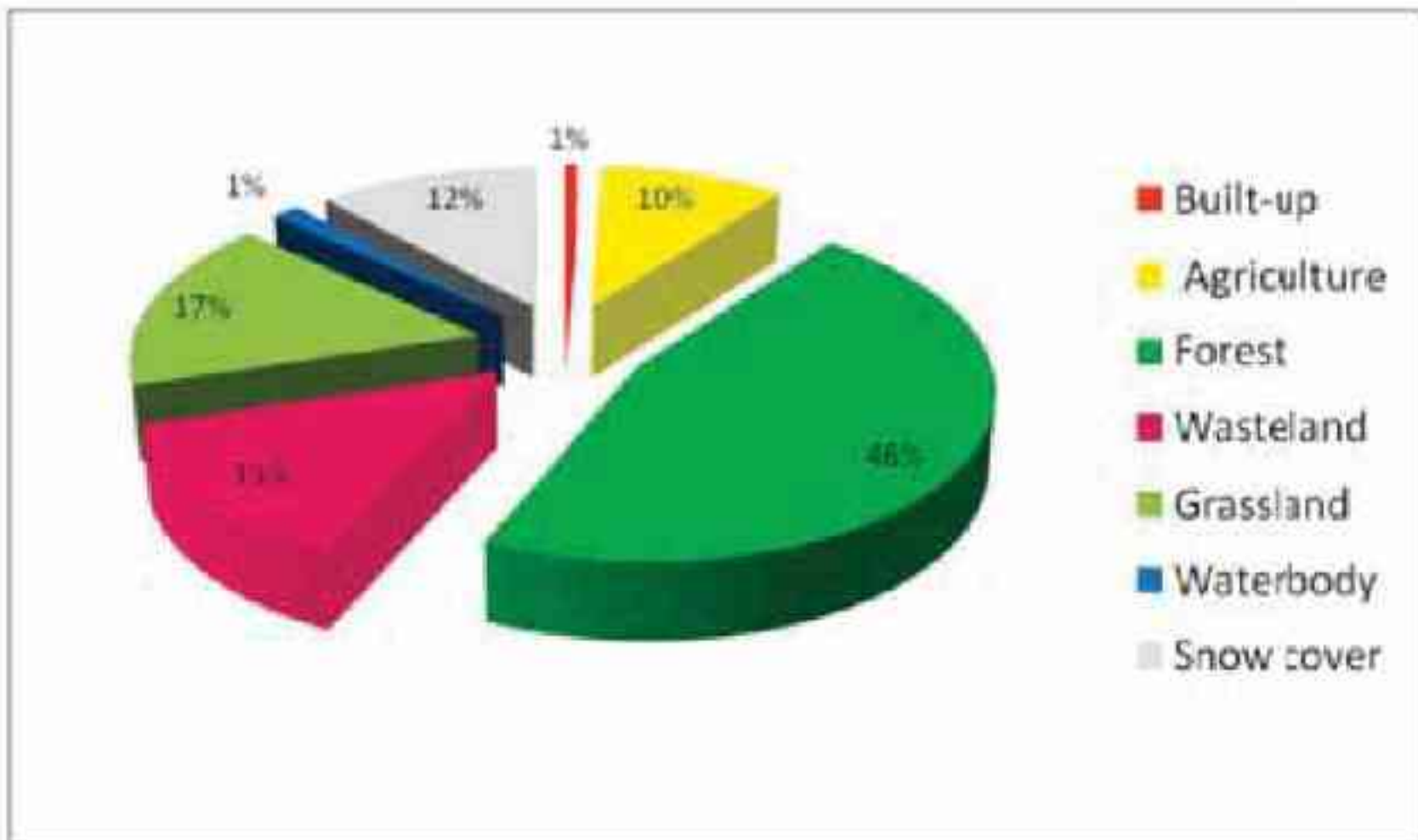
Fig. 2b. Percentage area under different major land use categories in Chamba district for the year 2015-16.
